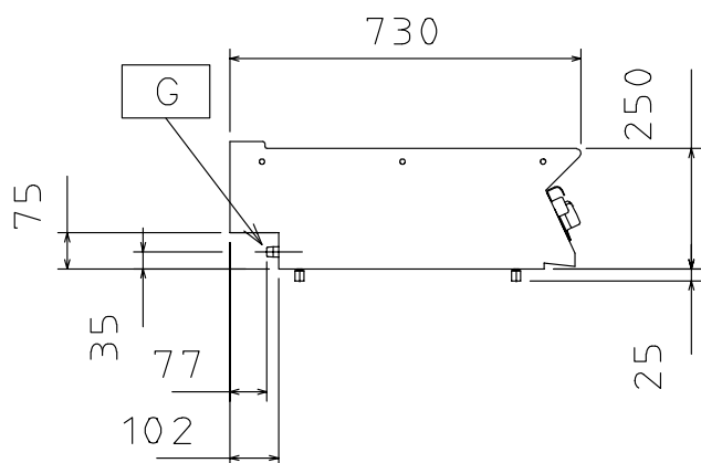
Lateral
